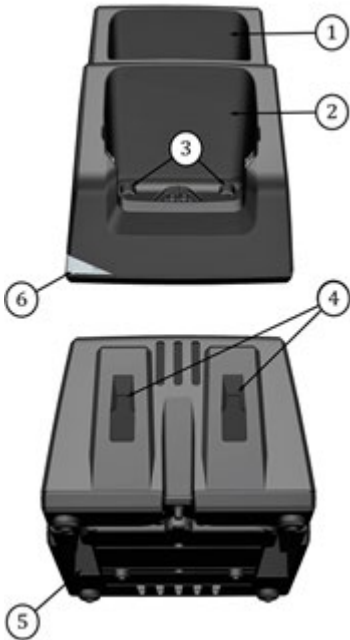
Figure 9 RCH-30 battery charger components
